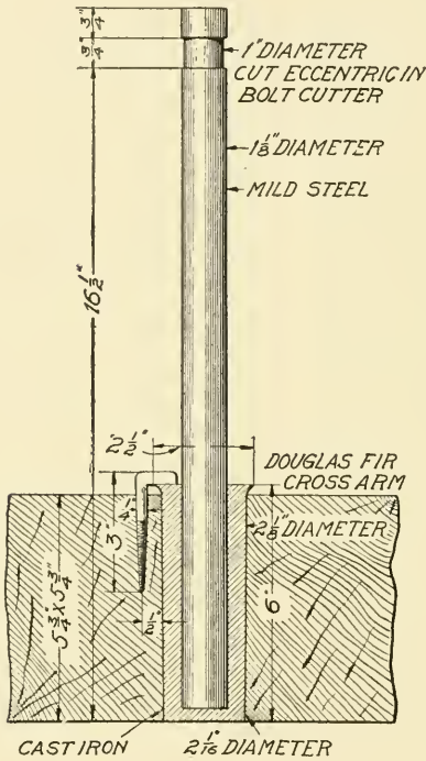
Fig. 42. Iron Pin Showing Dimensions
